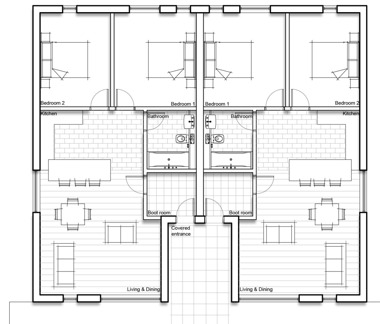
Proposed Ground Floor Plan Holiday Lets 3&4 1:100
