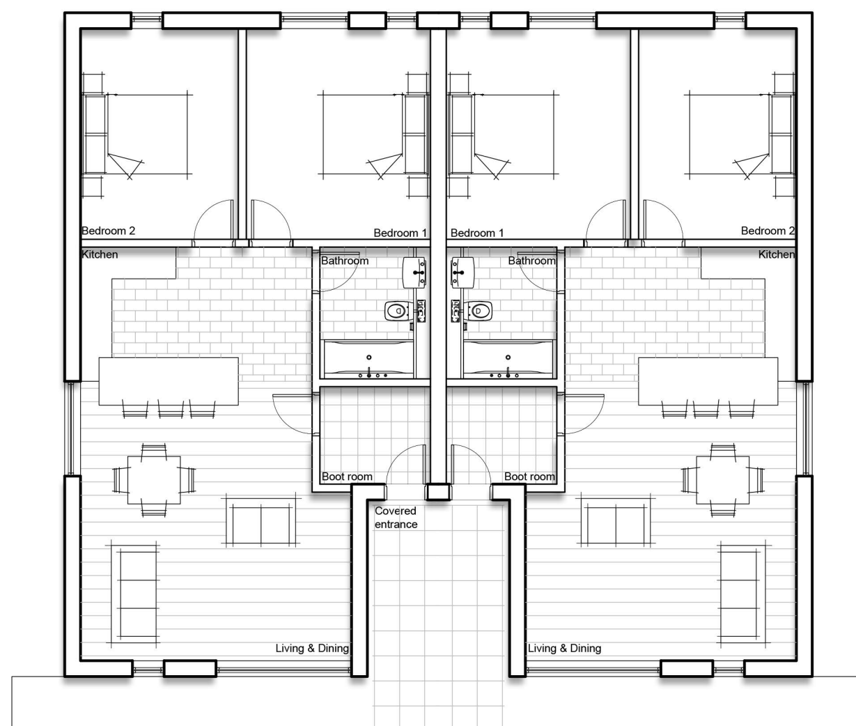
Proposed Ground Floor Plan Holiday Lets 1&2 1:100
